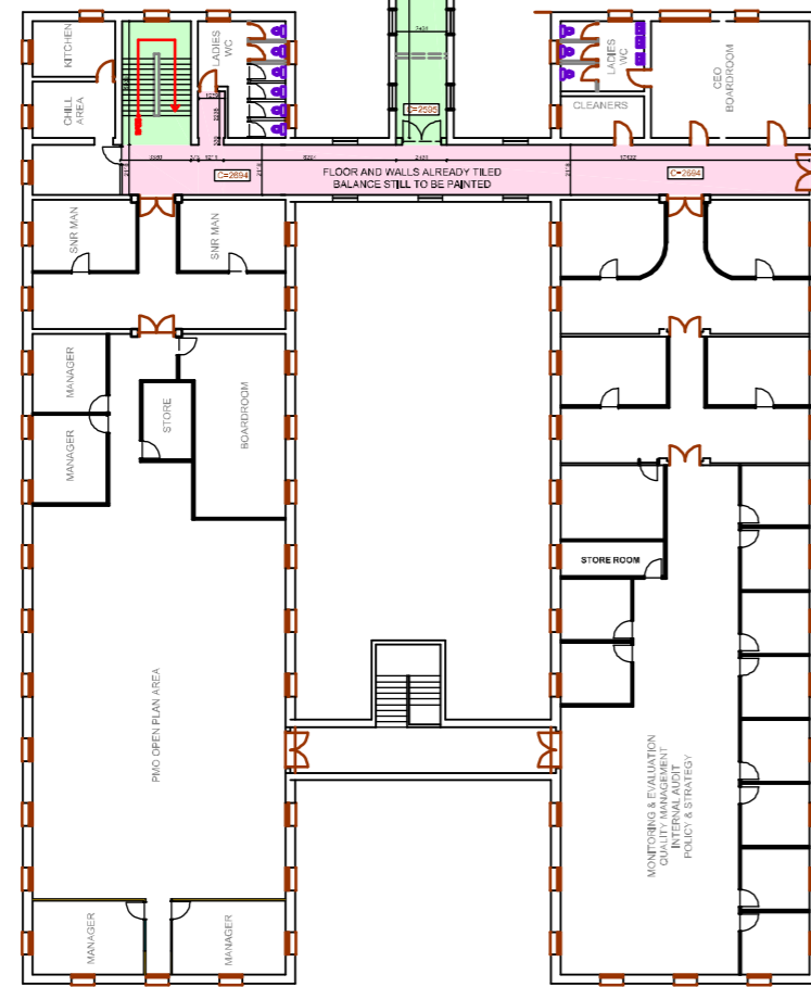
BLOCK E SECOND FLOOR PLAN
