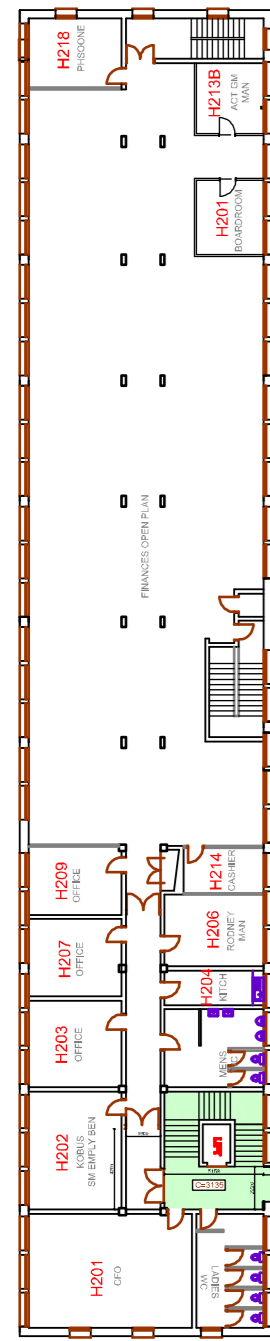
BLOCK H SECOND FLOOR PLAN
